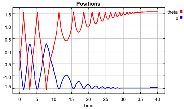
Fig. 3. A Zeno execution of the pendulum on a cart—displacements \theta and x vs time.
