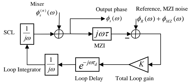
Fig. 2. Small signal phase propagation in the phase-lock loop.
