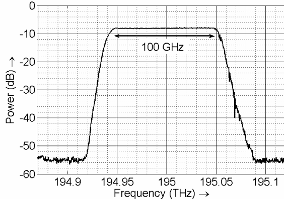
Fig. 5. Measured optical spectrum of the swept-frequency phase-locked SCL. RBW = 10 GHz
