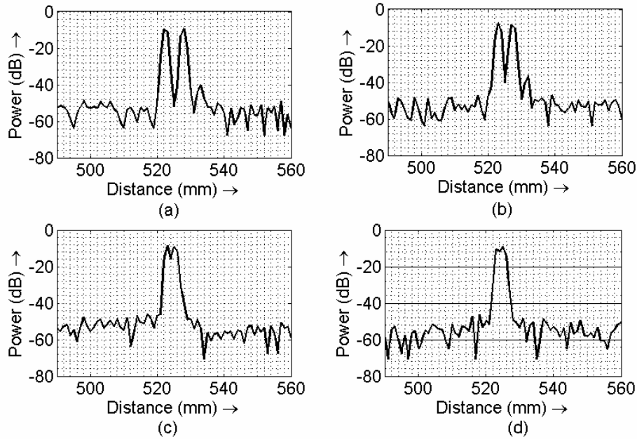
Fig. 7. Range resolution measurements using the swept-frequency SCL. The target was an acrylic sheet of refractive index 1.5 and thickness (a) 5.44 mm, (b) 4.29 mm, (c) 2.25 mm and (d) 1.49 mm.
