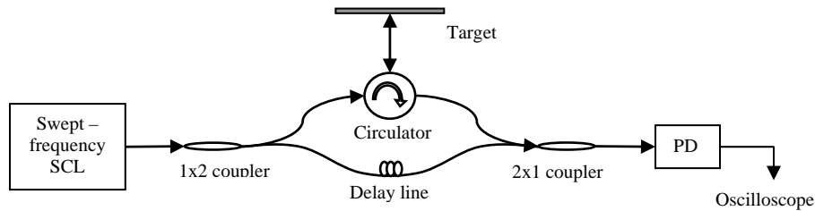
Fig. 6. Schematic of the ranging experiment with a linearly chirped optical source. PD: Photodetector
