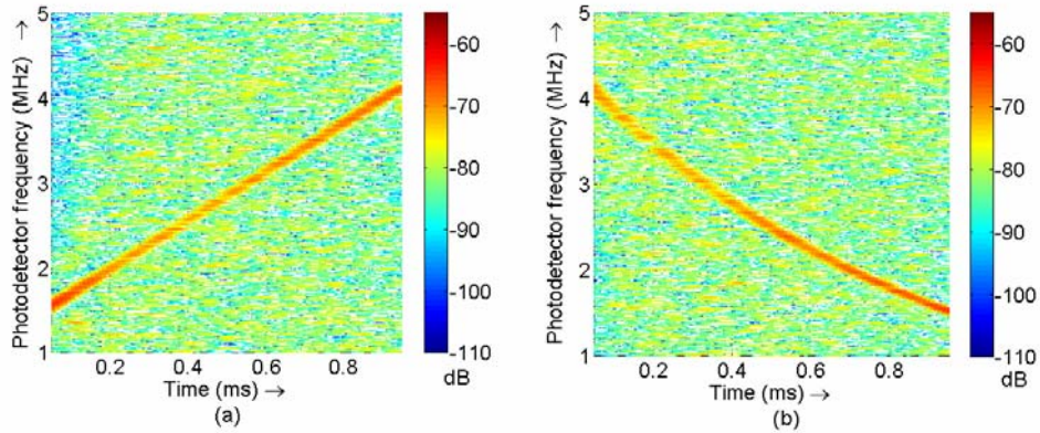
Fig.8. Measured spectrograms of the output of the loop photodetector, illustrating arbitrary sweeps of the SCL frequency. (a) The reference signal is swept linearly with time. (b) The reference signal is swept exponentially with time. The laser sweep rate varies between 50 GHz/ms and 150 GHz/ms.
