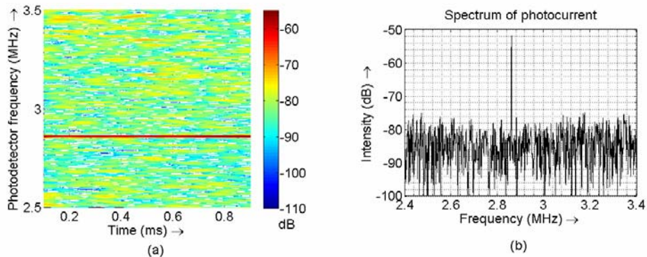
Fig.4. (a) Measured spectrogram of the output of the loop photodetector when the loop is in lock, corresponding to an optical sweep rate of 100 GHz/ms. (b) Fourier transform of the photodetector output measured over a 1 ms duration.
