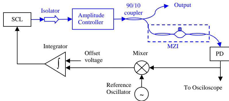
Fig. 1. Optoelectronic phase-lock loop for the generation of accurate broadband linear chirps. The optical path is shown in blue.
